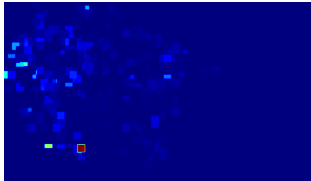
Attention Heatmap
